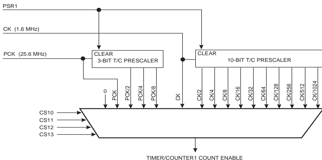
Figure 13-1. Timer/Counter1 Prescaler
